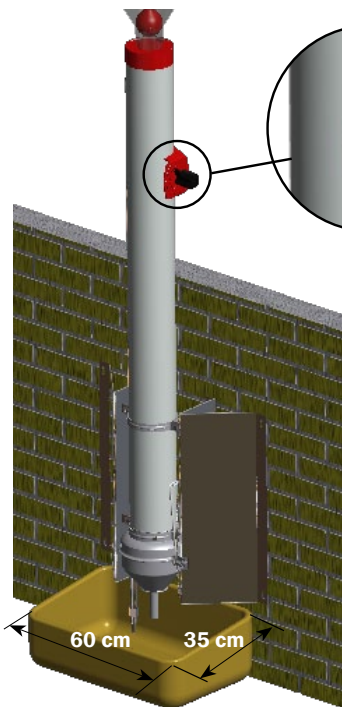
0227-495 COMBI-feeder, complet
